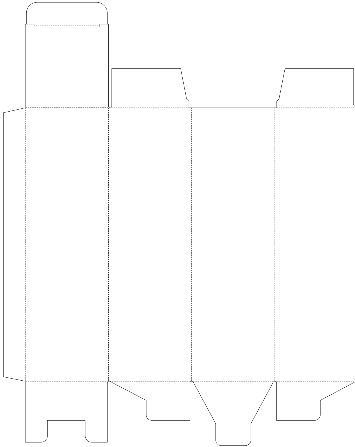
OPTIONAL BOX 250 x 76 x 76 mm SCALE (1:2)
